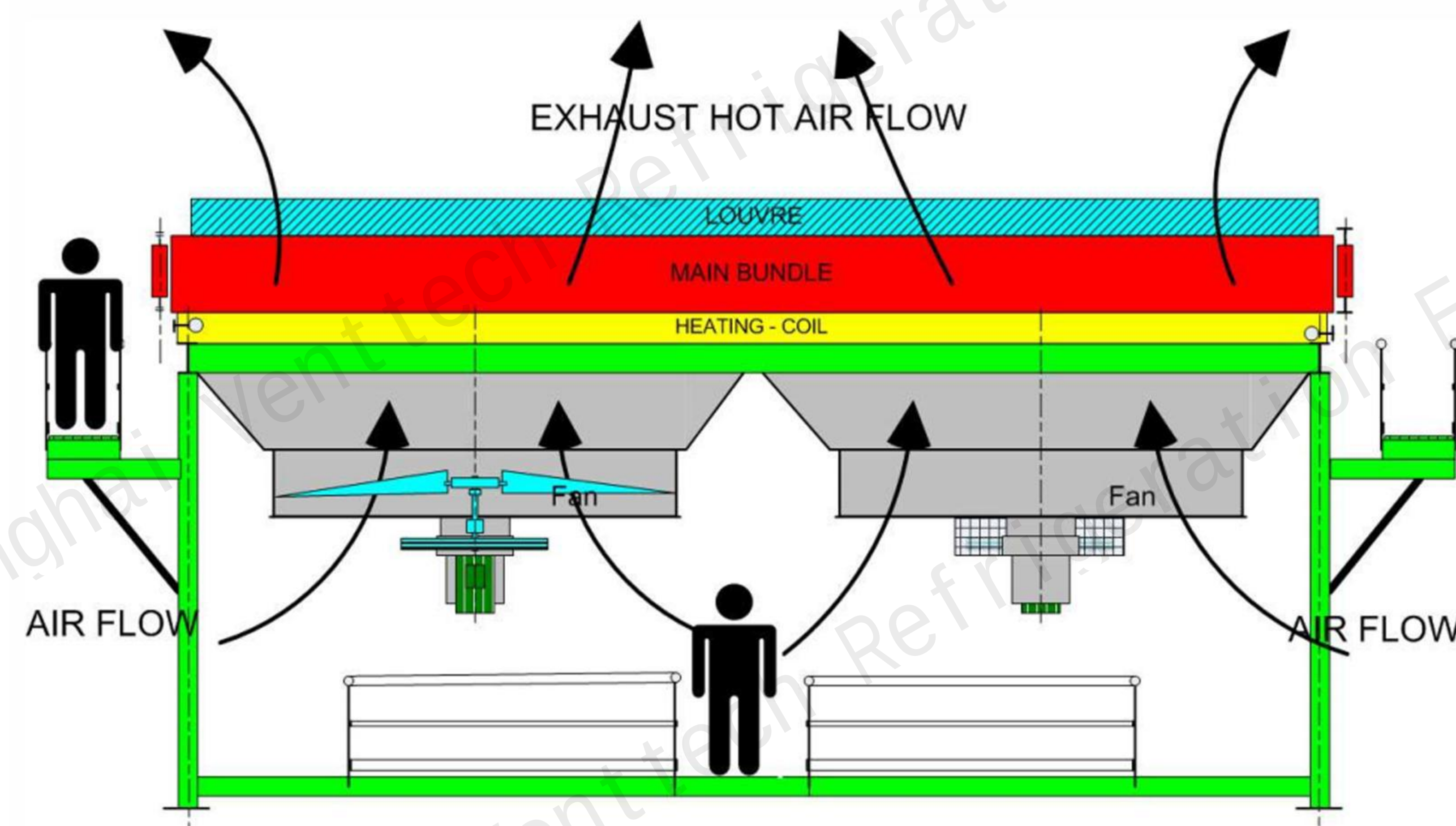
Forced Type
