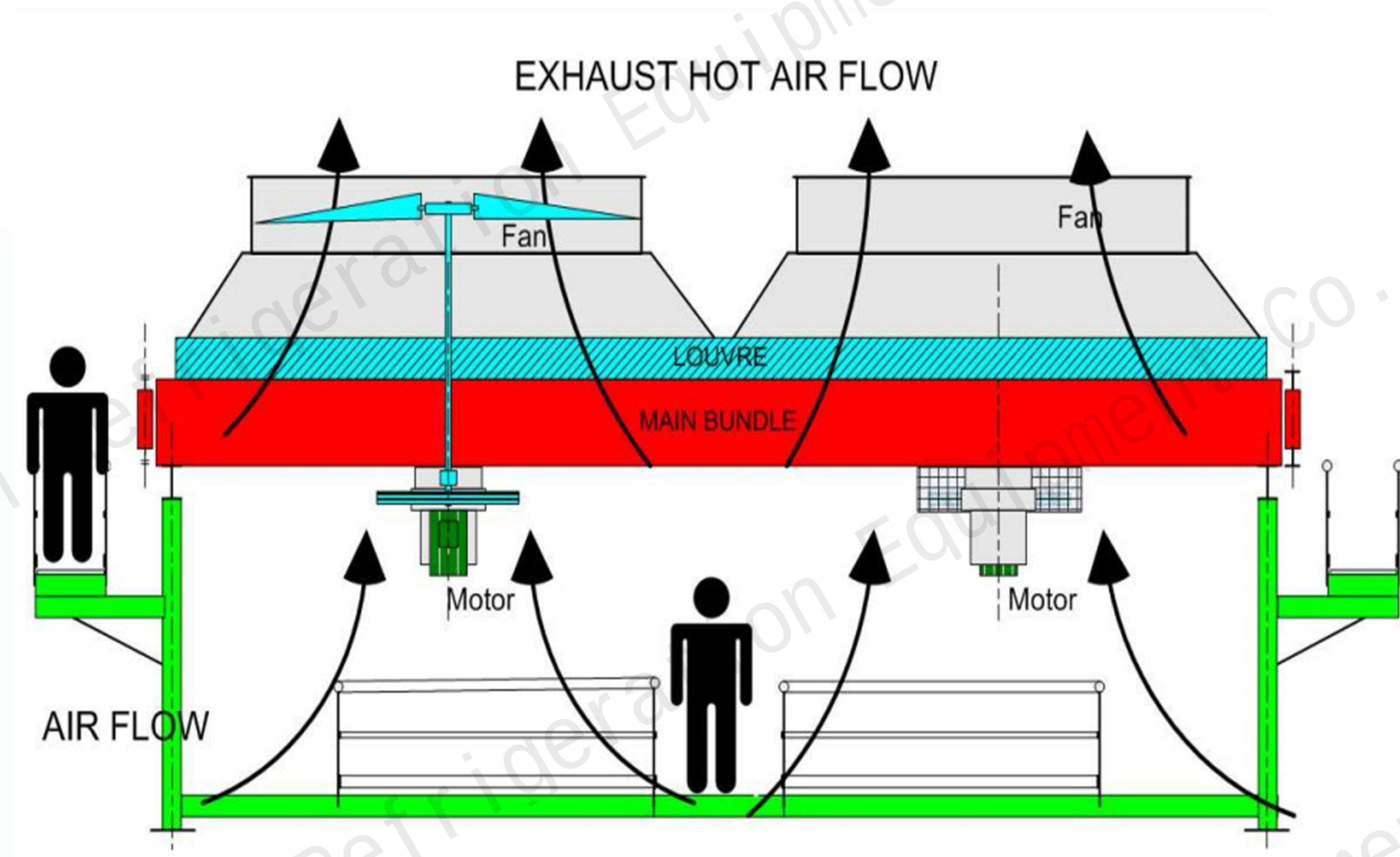
Induced Type
