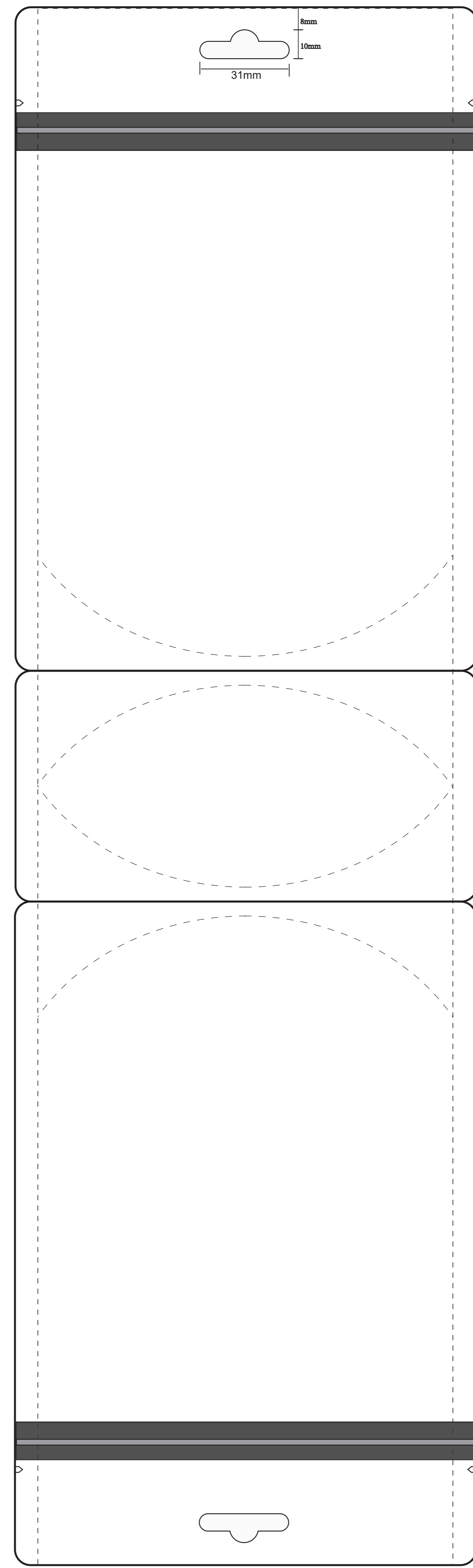
Dieline of ziplock stand up pouch
