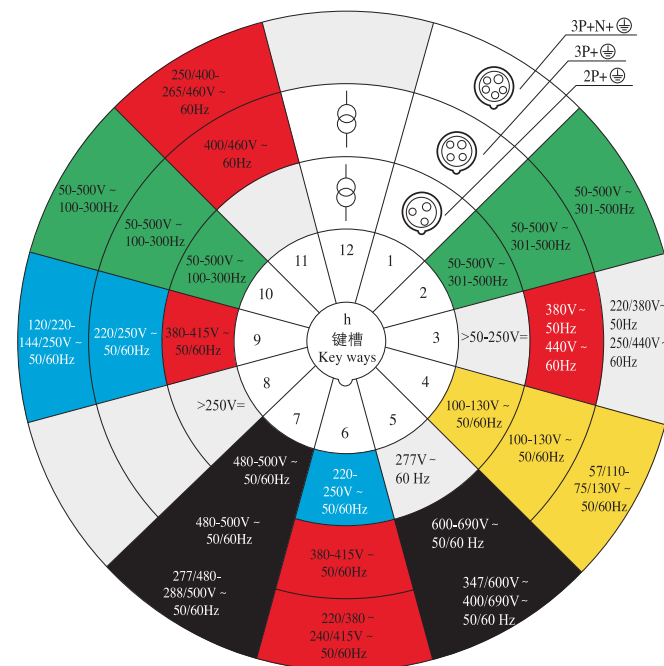
插座(前视图) SOCKET(front view)
