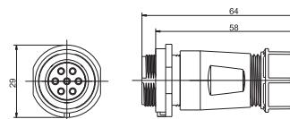
电缆对接插座 In-line cable connector
