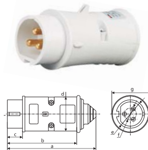
IP44 CEE/IEC 低压插头 32A
