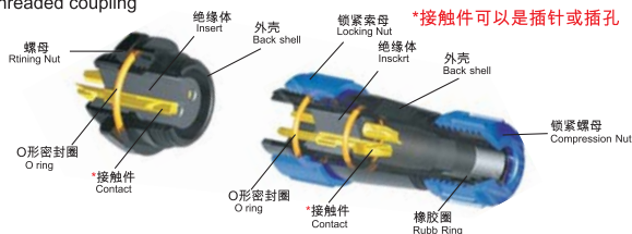
IP 68 Threaded coupling
