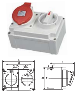
IP44 CEE/IEC 机械联锁 16A
