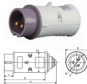
IP44 CEE/IEC 低压插头 16A
