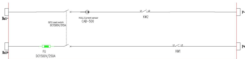
Main Wiring Diagram of High-voltage Box
