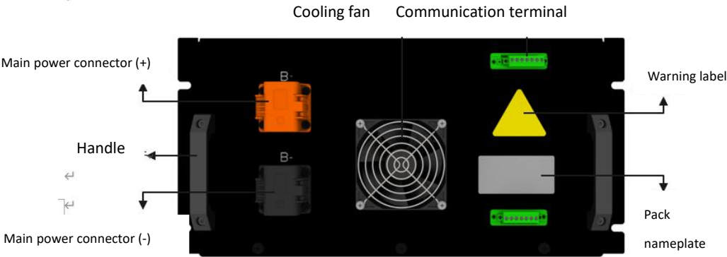
Schematic Diagram of B-PACK Panel:
