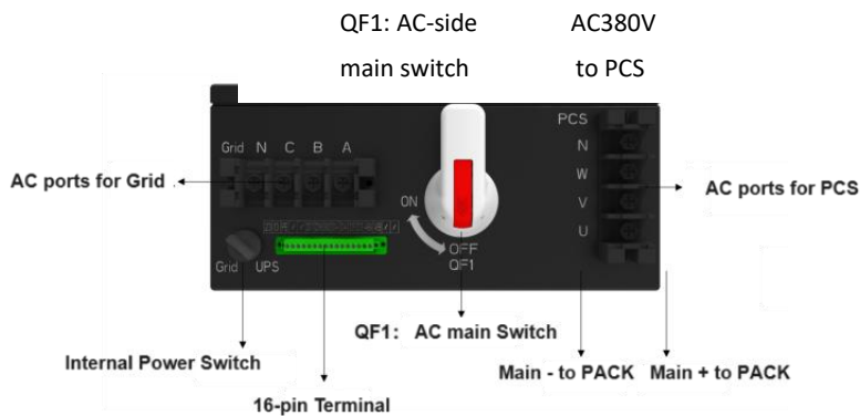
Schematic Diagram of Rear Panel Layout of Control Box:
