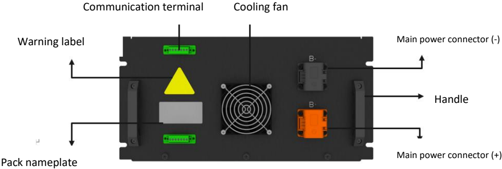
Schematic Diagram of A-PACK Panel:
