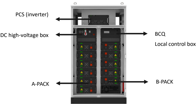
Layout of ECO-E100WX
