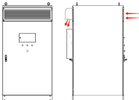
Figure 4-2 ECO-E150WS Air inlet and Outlet
