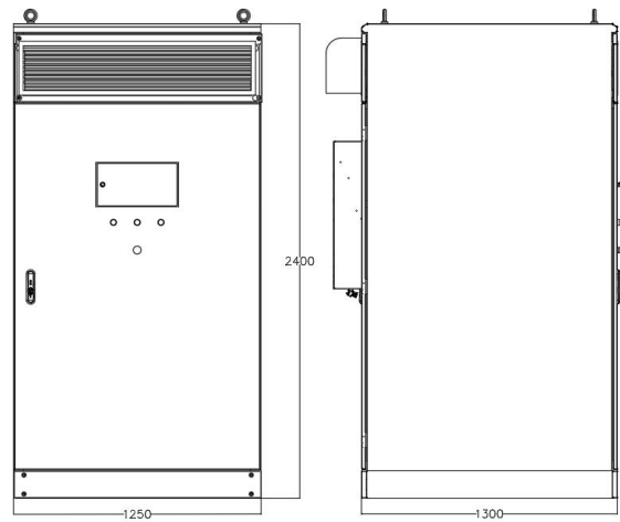
Figure 4-1 ECO-E150WS Dimensions
