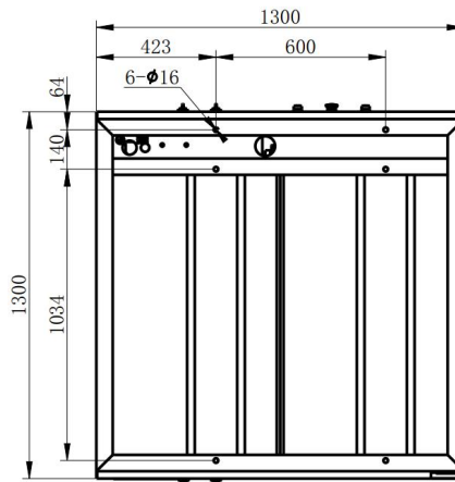
Figure 4-4 Base layout of the Cabinet
