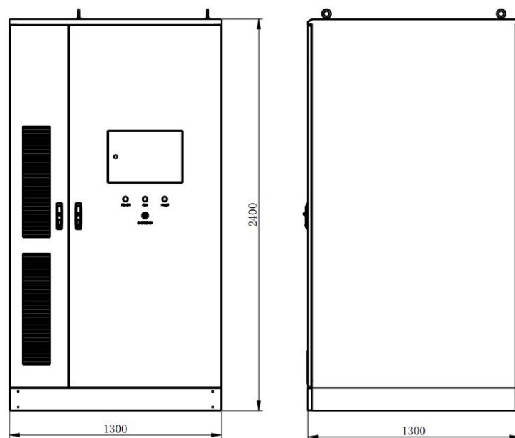
Figure 4-1 ECO-B372LS Dimensions
