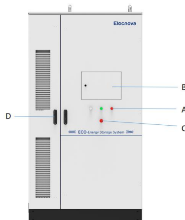
Figure 3-2 Appearance
