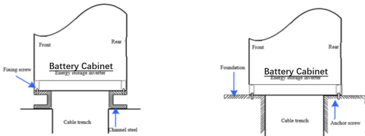
Figure 5-7 Fixing Method for Battery Cabinet
