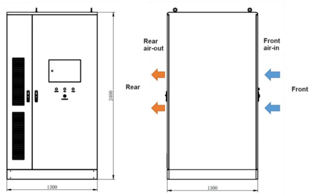
Figure 4-2 ECO-B372LS Air inlet and Outlet
