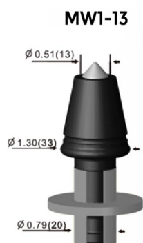
Concrete Pick Medium&Large Milling Machine
