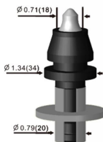
Asphalt Pick Medium&Large Milling Machine
