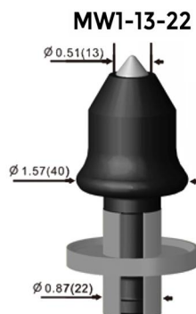
Concrete Pick Ø22mm Large Milling Machine
