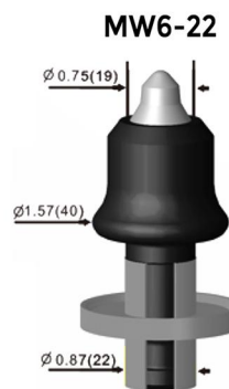
Asphalt Pick Stabilizers Recyclers
