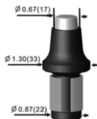
Scarifier Blades Pick Competitive blade systems
