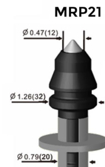
Concrete Pick Medium&Large Milling Machine
