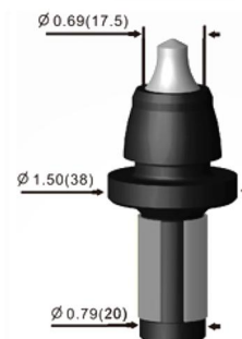
Asphalt Pick All Type Milling Machine
