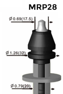
Asphalt Pick Medium&Large Milling Machine
