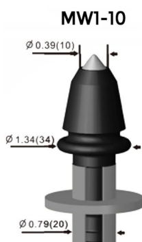
Concrete Pick Small Milling Machine
