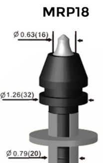
Asphalt Pick Small Milling Machine
