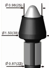
Scarifier Blades Pick All Types of road surfaces
