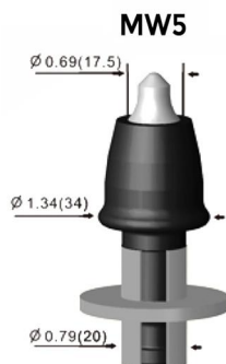
Asphalt Pick Medium&Large Milling Machine
