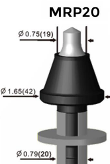
Asphalt Pick Medium&Large Milling Machine
