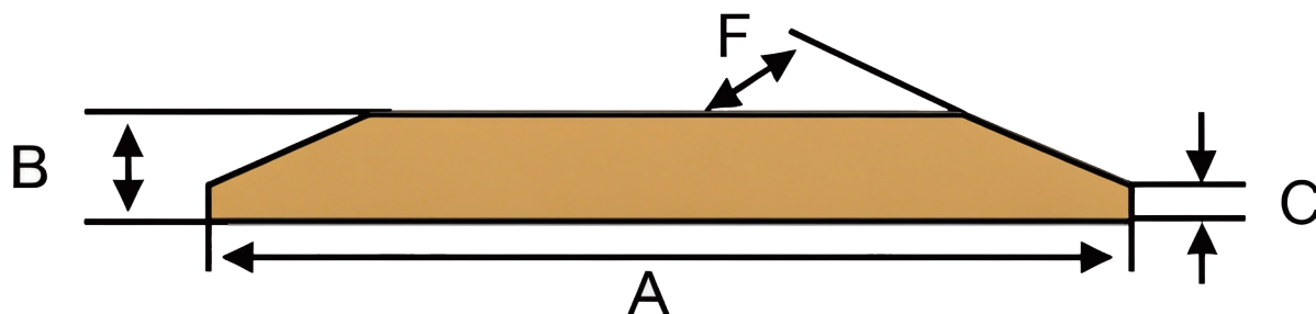
Double Bevel Flat Profile
