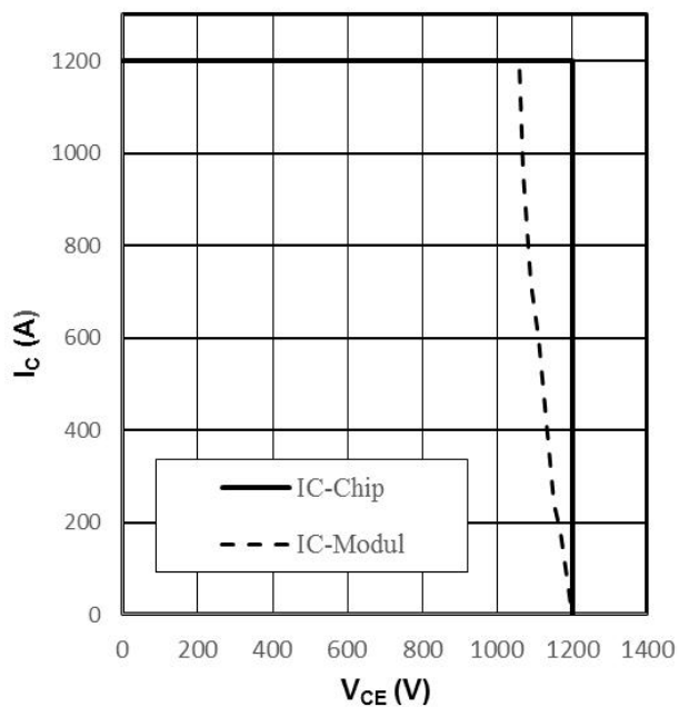
Fig 7. reverse bias safe operating area IGBT, I_C=f(V_{CE}) , V_{GE}=\pm 15V , R_{Goff}=1.1\Omega , T_{vj}=125^\circ C
