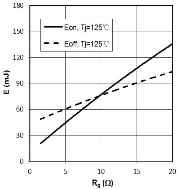
Fig 5. switching losses IGBT, E_{on}=f(R_g) , E_{off}=f(R_g) , V_{GE}=\pm 15V , I_C=600A , V_{CE}=600V
