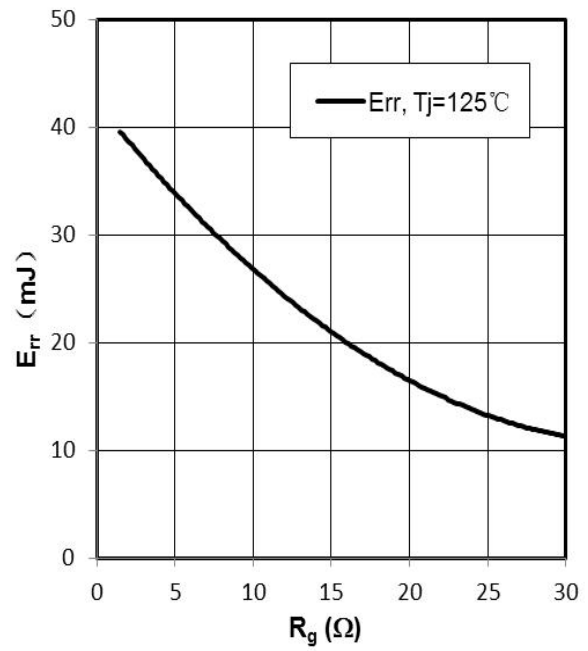
Fig 10. switching losses Diode, E_{rr}=f(R_g) , I_F=600A , V_{CE}=600V
