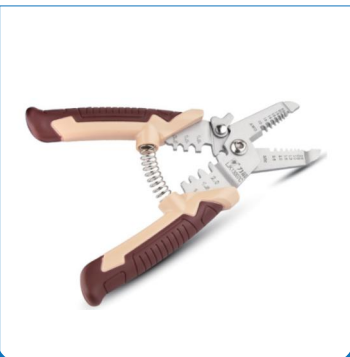
7" Multipurpose wire stripper ◆ AWG10-12-14-16-18-20-22
