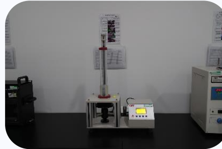
Falling ball rebound detector
