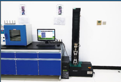
老化 and 压缩永久变形测试仪 Aging and compression permanent deformation tester
