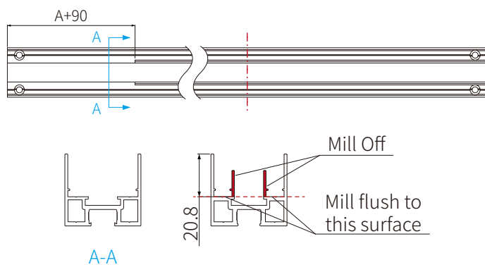
40 Door Upper/Bottom Frame Processing Drawing
