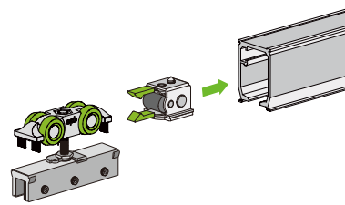
无需开孔 no need to hole
