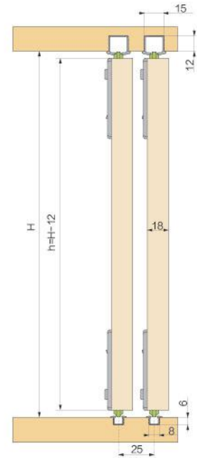
阻尼单轨02 SINGLE TRACK FOR SOFT CLOSE 02
