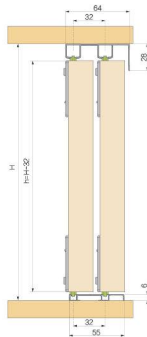
双轨道25mm DOUBLE TRACK FOR 25mm
