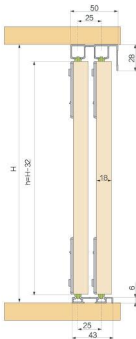
双轨道18mm DOUBLE TRACK FOR 18mm
