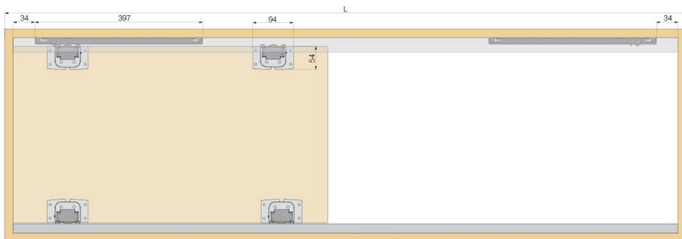
双轨道18mm DOUBLE TRACK FOR 18mm
