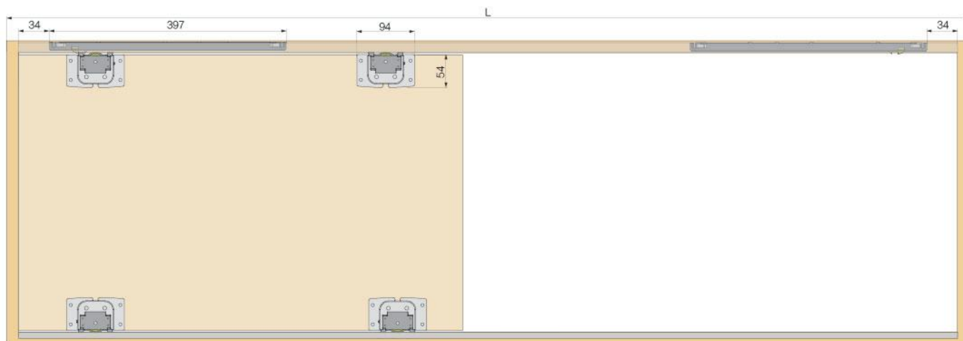
阻尼单轨02 SINGLE TRACK FOR SOFT CLOSE 02
