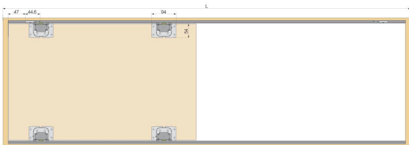
普通单轨 SINGLE TRACK
