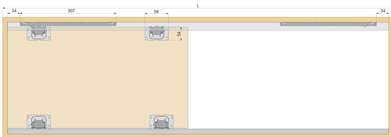
双轨道25mm DOUBLE TRACK FOR 25mm
