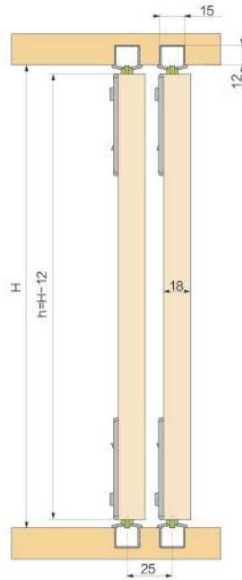
阻尼单轨01 SINGLE TRACK FOR SOFT CLOSE 01
