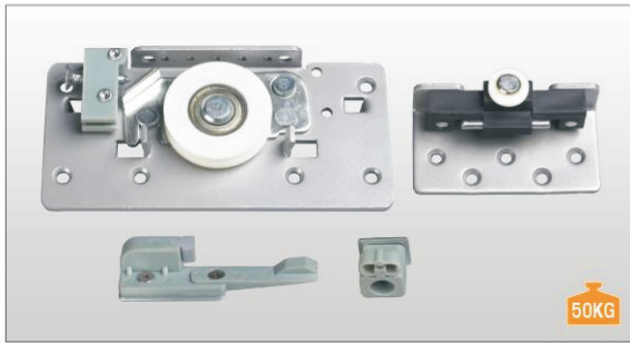
OPK-30143 Top Hang System-Inner Door
