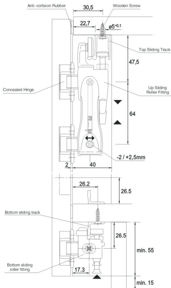
Folding Door Installation Sizes & Right View
