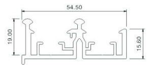
CFG-789-01 Color: Champagne / Silver
