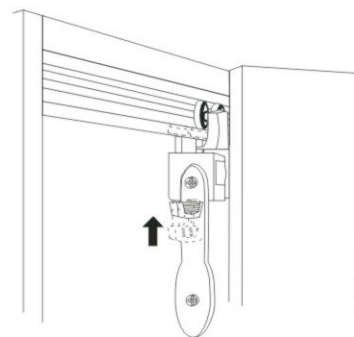
5. Push Up Roller Guide, Make Up Roller Into Up Sliding Track
