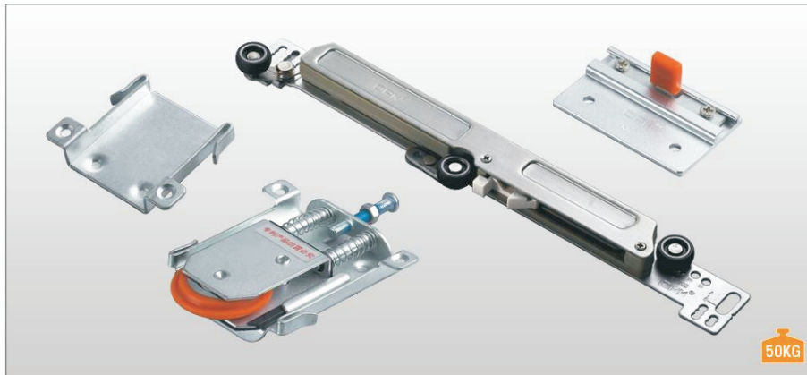
OPK-60302B-03 Soft Closing Mechanism
