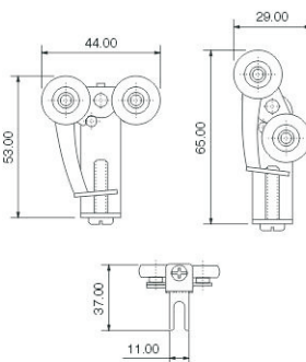
OPK-ZJ-B03 Manual-adjustable Up Roller
