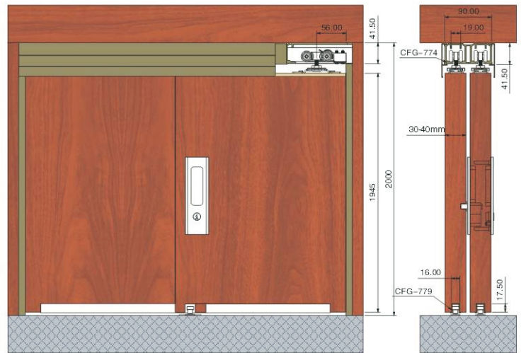
CFA-115 Sliding Steel-Wood-Composite Door Hanging Roller
