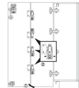
3. Hinge & Flush Bolt Installation
