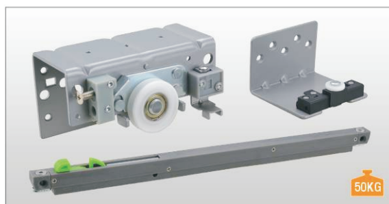
CFD-446A Top Hang System–outer Door With Soft Close
