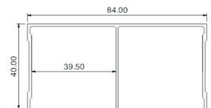
CFG-789-01 Color: Champagne / Silver
