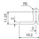
CFG-787-01 Color: Champagne / Silver
