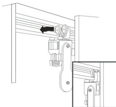
4. Put The Up Roller Into Up Sliding Track
