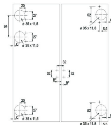
1. Hinge Hole Sizes And Situations
