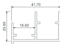
CFG-787-02 Color: Champagne / Silver
