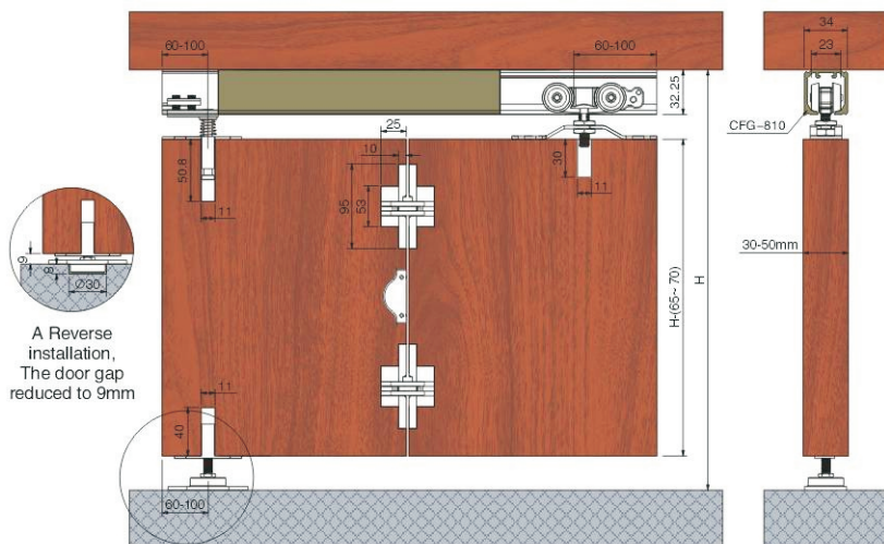
CFC-337 Sliding Folding Door Hanging Roller
