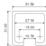
CFG-813-01 Color: Champagne / Silver
