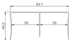
LT E047 Up Track 0.6kg/m \delta = 1.0\text{mm}
