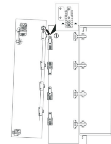
2. Hinge Connecting
