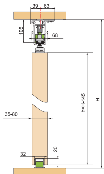
带阻尼 With Damping
