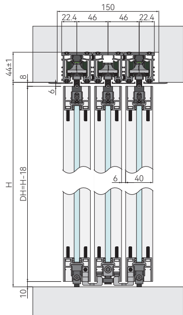
CONCEALED MOUNTING
