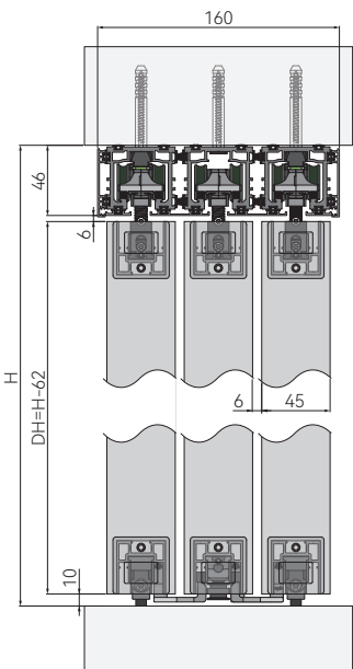
SURFACE MOUNTING
