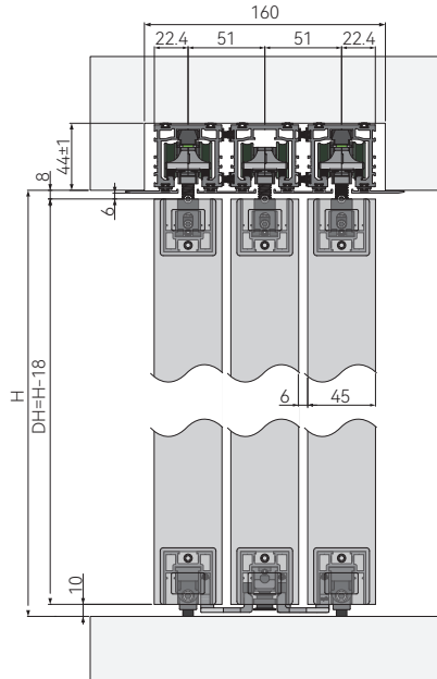
CONCEALED MOUNTING
