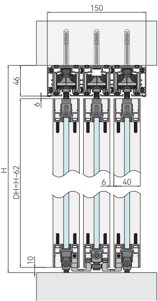
SURFACE MOUNTING
