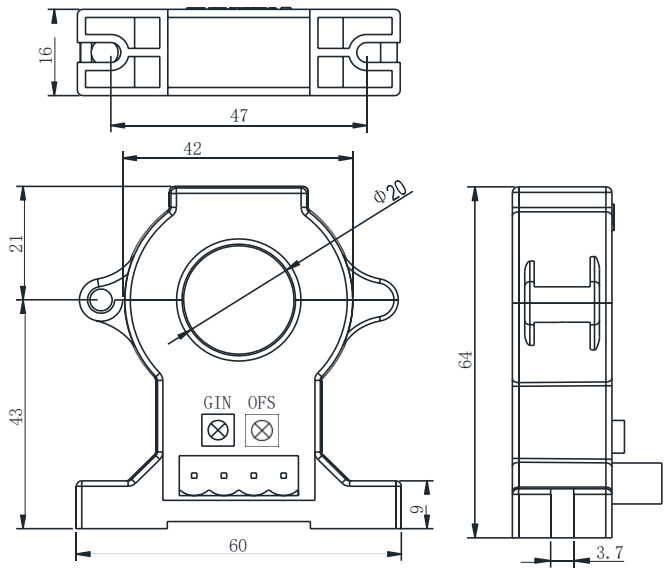
AHKC-EKA (50A/5V) aperture Φ20mm
