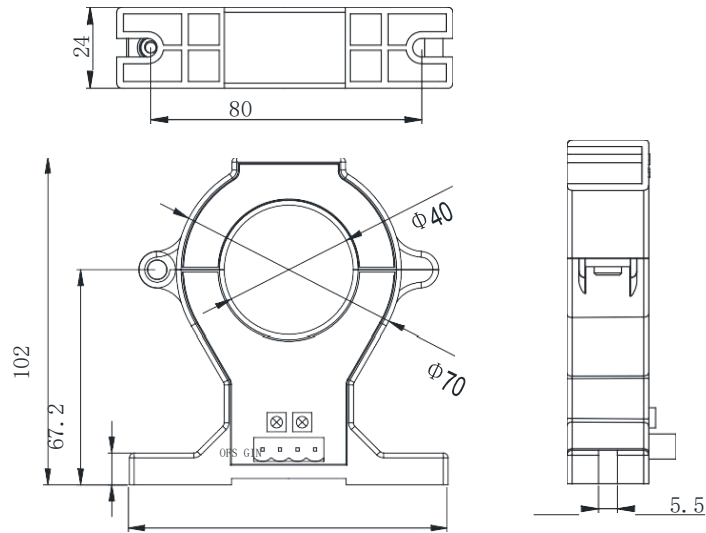
AHKC-EKB (100A/5V) aperture Φ40mm
