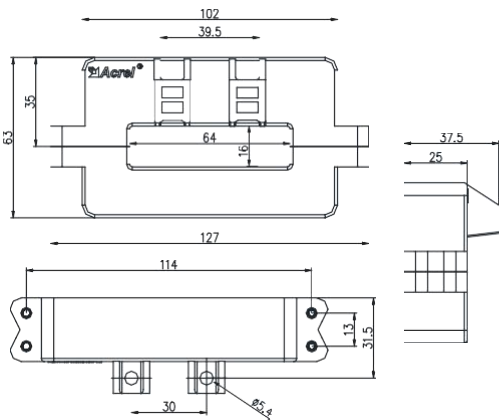
AHKC-K (200A/5V) aperture Φ64*16mm
