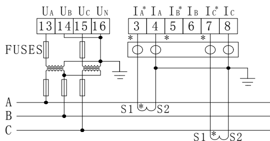
三相三线2PT、2CT Three-phase 3-wire 2PT, 2CT
