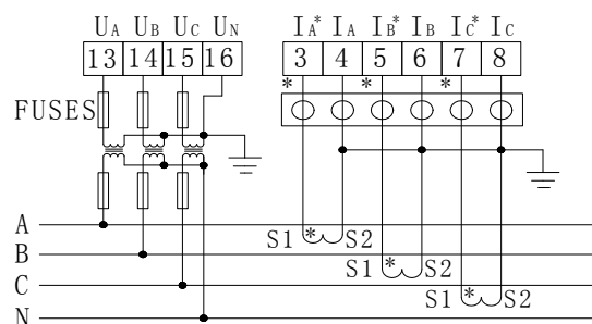
三相四线3PT、3CT Three-phase 4-wire 3PT, 3CT
