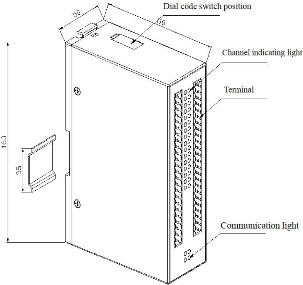
ARTU-K8/K16/K32 Remote signal unit Outline and dimensions
