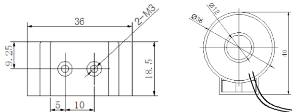
Figure 3 Dimension of transformer (ADW350WA 20(100)A)
