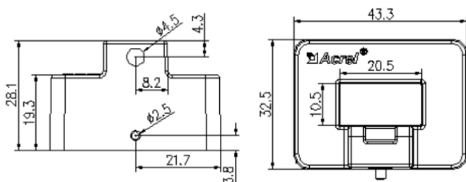
Figure 4 Dimension of Hall current sensor AHKC-BS (ADW350WD)
