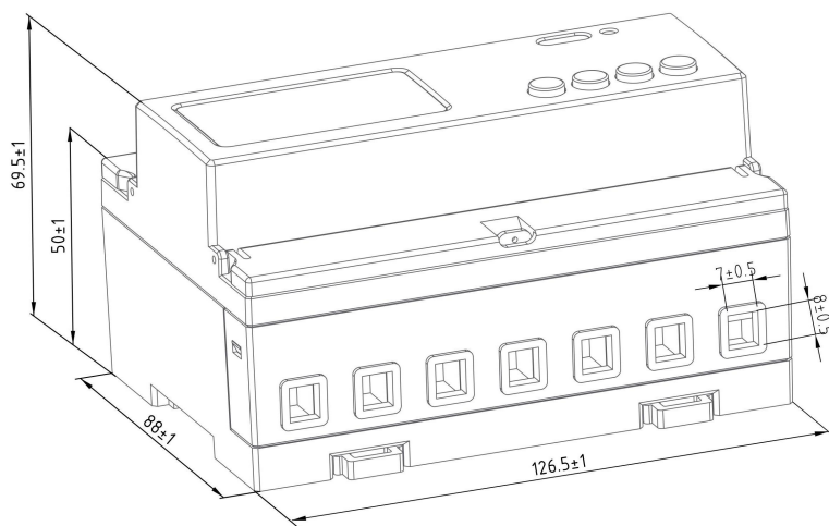
Fig2 direct connect
