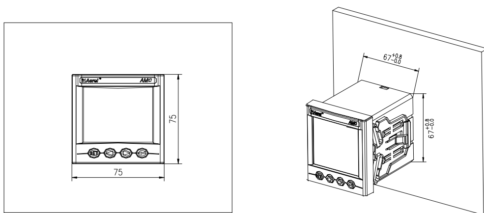
Figure 3 AMC72 installation dimensions
