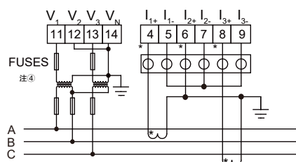
3P3W/2PT+2CT-2(Meter is set to 3P3W-3CT) Note③
