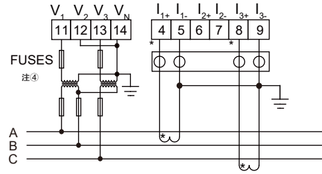
3P3W/2PT+2CT-1(Meter is set to 3P3W-2CT)
