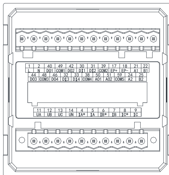
Figure 8 APM510 extended K/2M/2C wiring diagram
