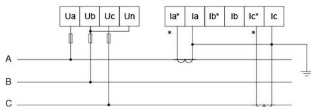
Three phase three lines connect via CT
