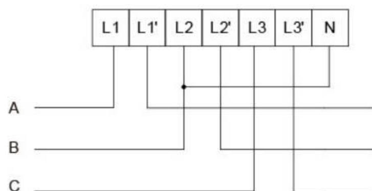
Three phase three lines direct connect
