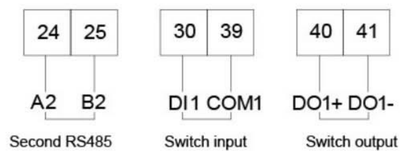
Communication, pulse connection
