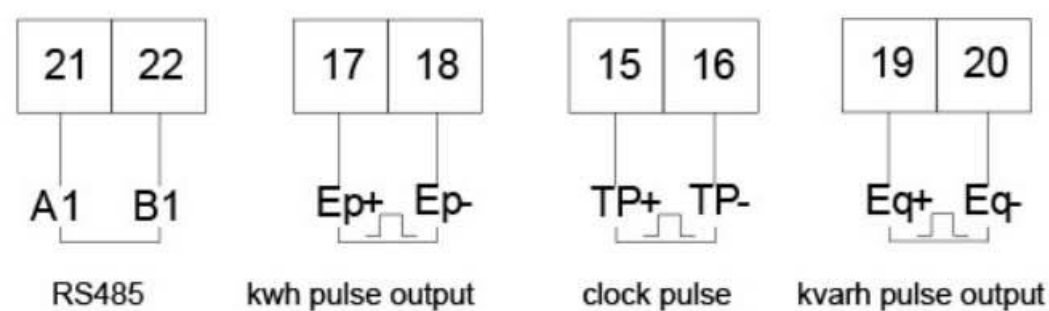
Communication, pulse connection
