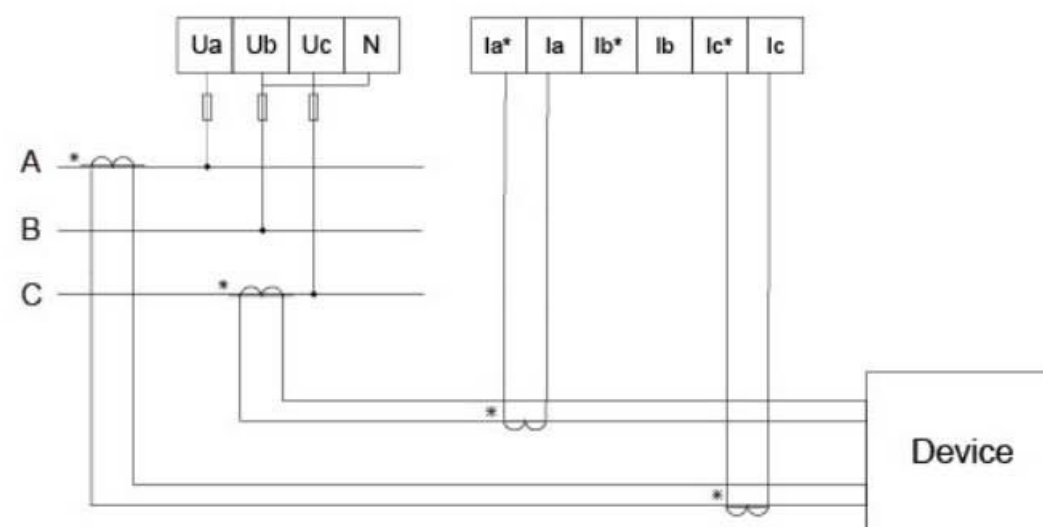
Three phase three lines, 2CT
