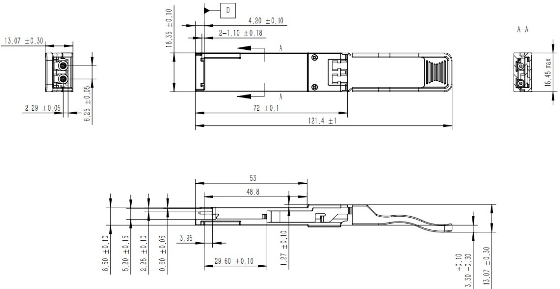
Figure 2. Mechanical dimensions
