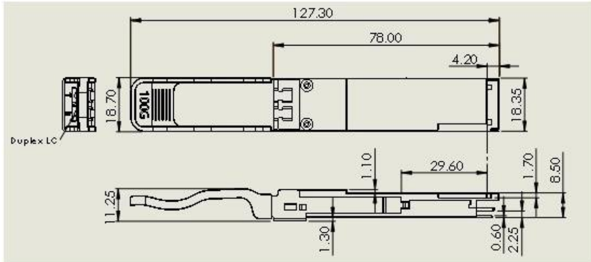
Figure 4. Mechanical Outline
