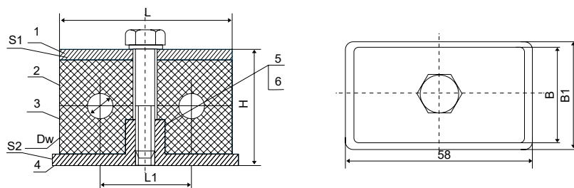
TD 型管子吊架基本尺寸 Basic size of TD type pipe hanger
