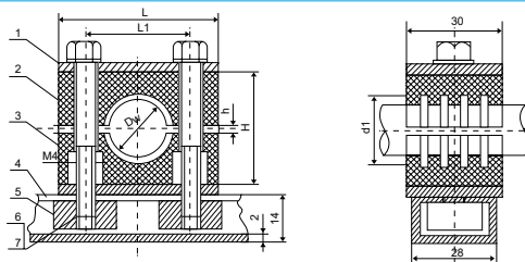
1- 压板; 2- 上本体; 3- 下本体; 4- 导轨; 5- 螺母; 6- 螺栓; 7- 垫圈 1-Pressing plate; 2-Upper body;3-Lower body;4- Rail; 5-Nut; 6-Bolt; 7-Washer
